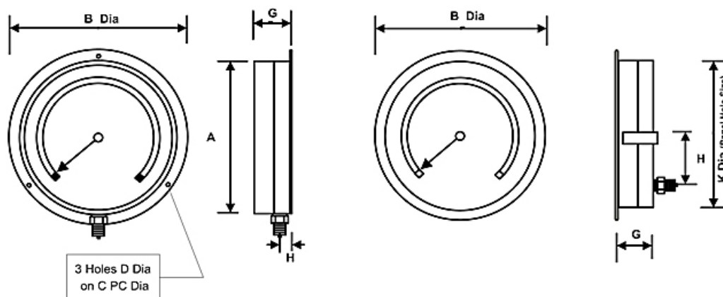
Direct / Surface Mounting
