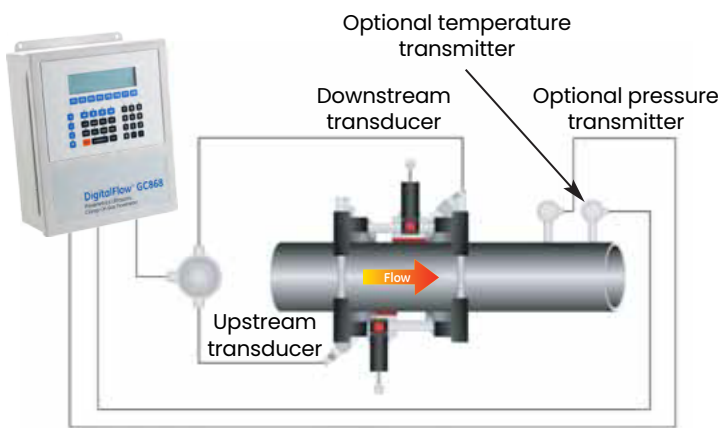
Typical meter set-up for standard volumetric
