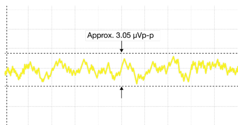
Noise waveform example at 0V output in 10 V output range (observed using a 1000 times amplifier with a 10 kHz band-limiting filter)
