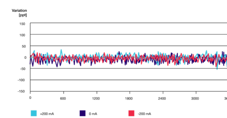
Example of 1 hour stability in output mA (As reference data)
